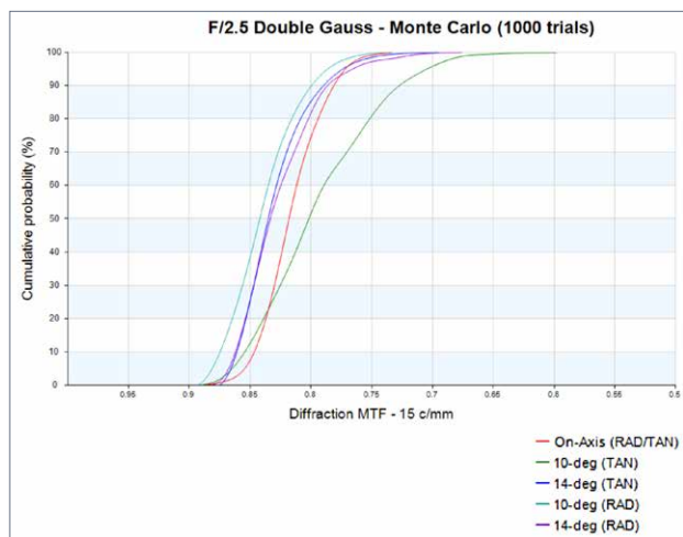
Figure 3: Monte Carlo cumulative probability chart
